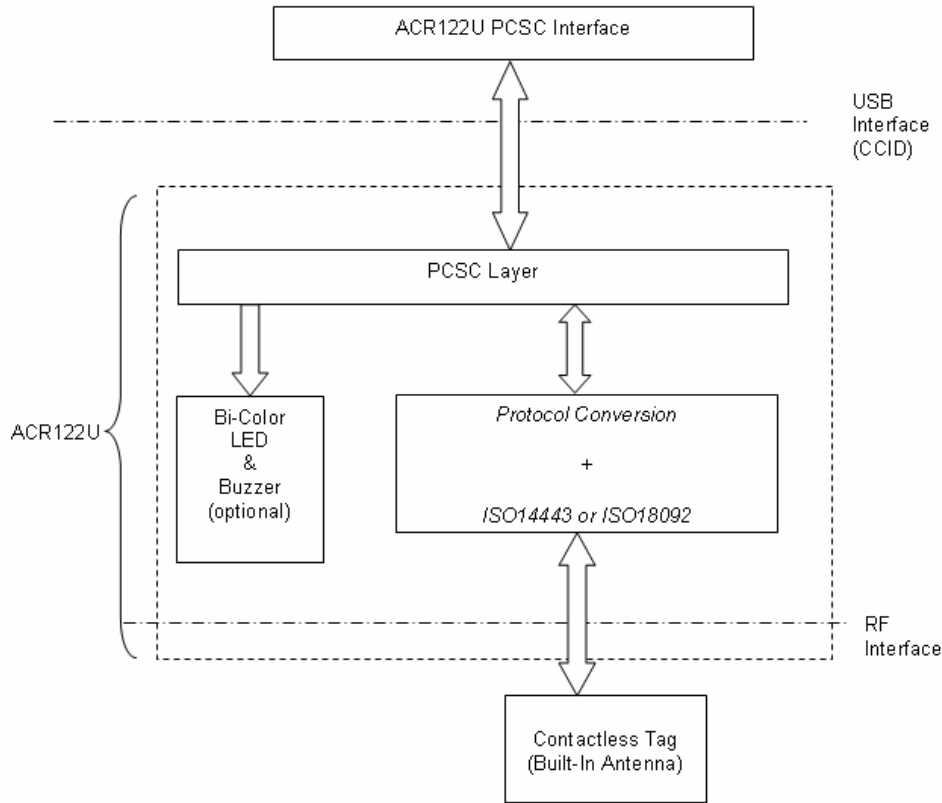
Figure 1: Communication Flow Chart of ACR122U
